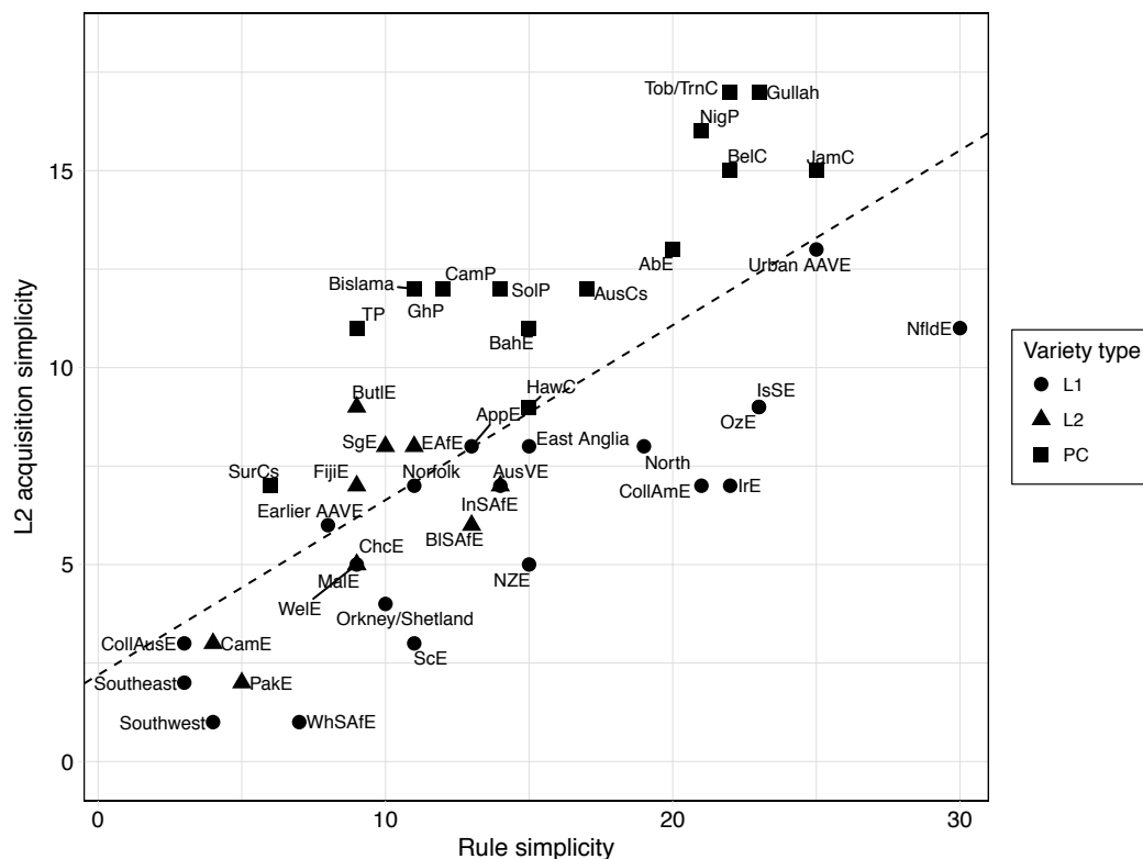
Figure 23.5. L2-simplicity by rule simplicity. The dotted trend line represents linear estimate of the relationship. (adapted from Kortmann & Szmrecsanyi 2009:Diagram 1)
