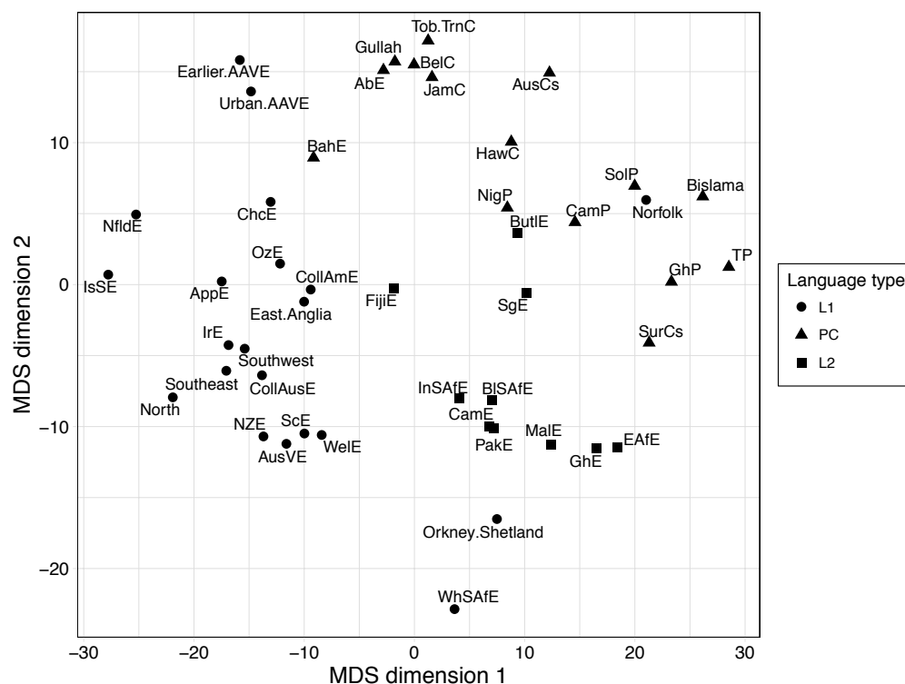
Figure 23.1. Metric Multidimensional Scaling (MDS) map, based on the morphosyntax survey coming with the Handbook of Varieties of English (see Kortmann & Szmrecsanyi 2004). Proximity between varieties in the plot is proportional to their aggregate morphosyntactic similarity. (See the appendix for a list of abbreviations.)
