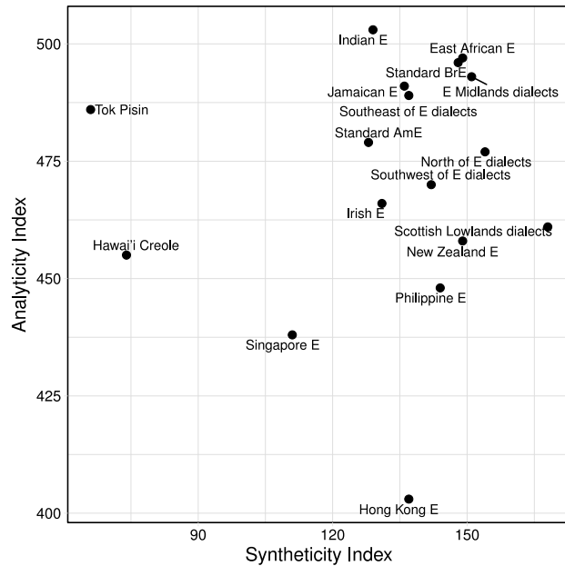
Figure 23.4. Tok Pisin and Hawai'i Creole vis-à-vis varieties of English: total number of analytic types against total number of synthetic types (focus on inventory sizes). (adapted from Siegel et al. 2014: Figure 2)
